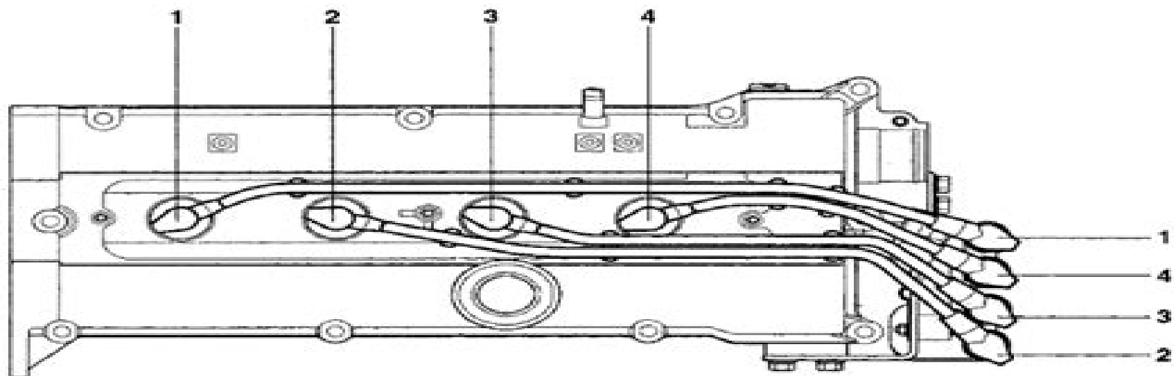
Fig 1: Routing Spark Plug Wires (4-Cylinder Engine)
