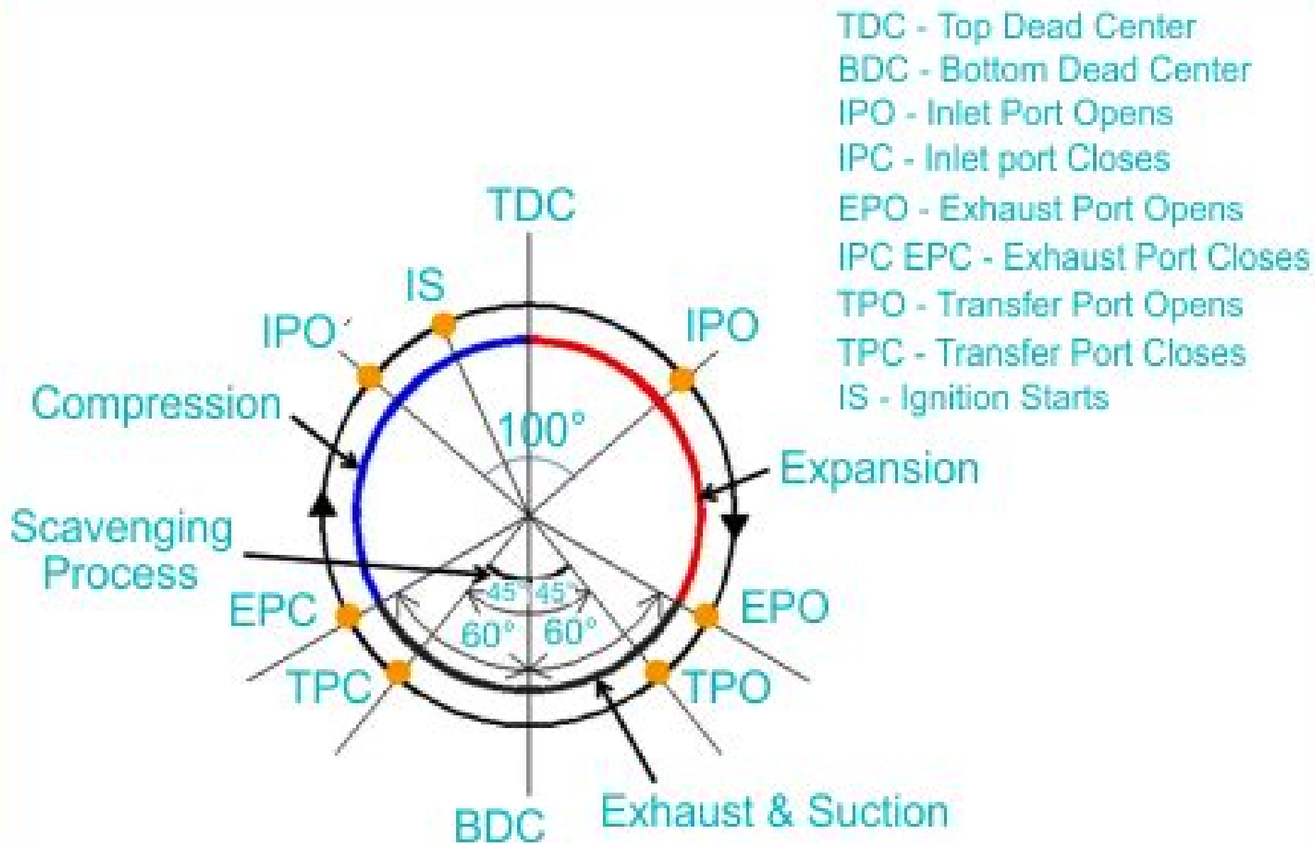
Valve Timing Diagram of 2 Stroke Petrol Engine
