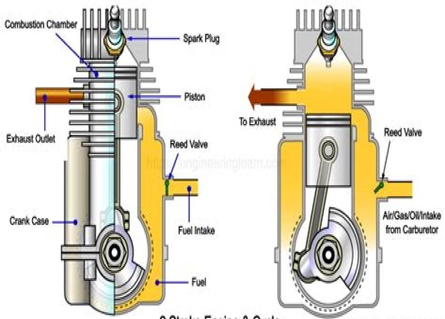
2 Stroke Engine & Cycle
