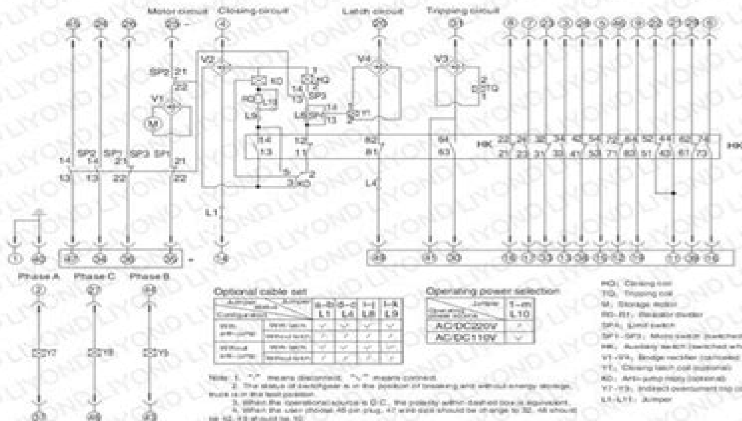
Drawing 4a The secondary wiring principle drawing of fixed type VCB
