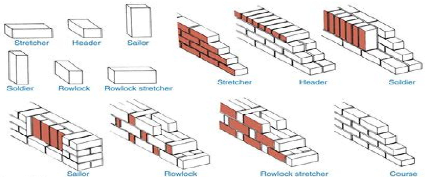
Figure 10-10. Names of brick positions in a wall.
