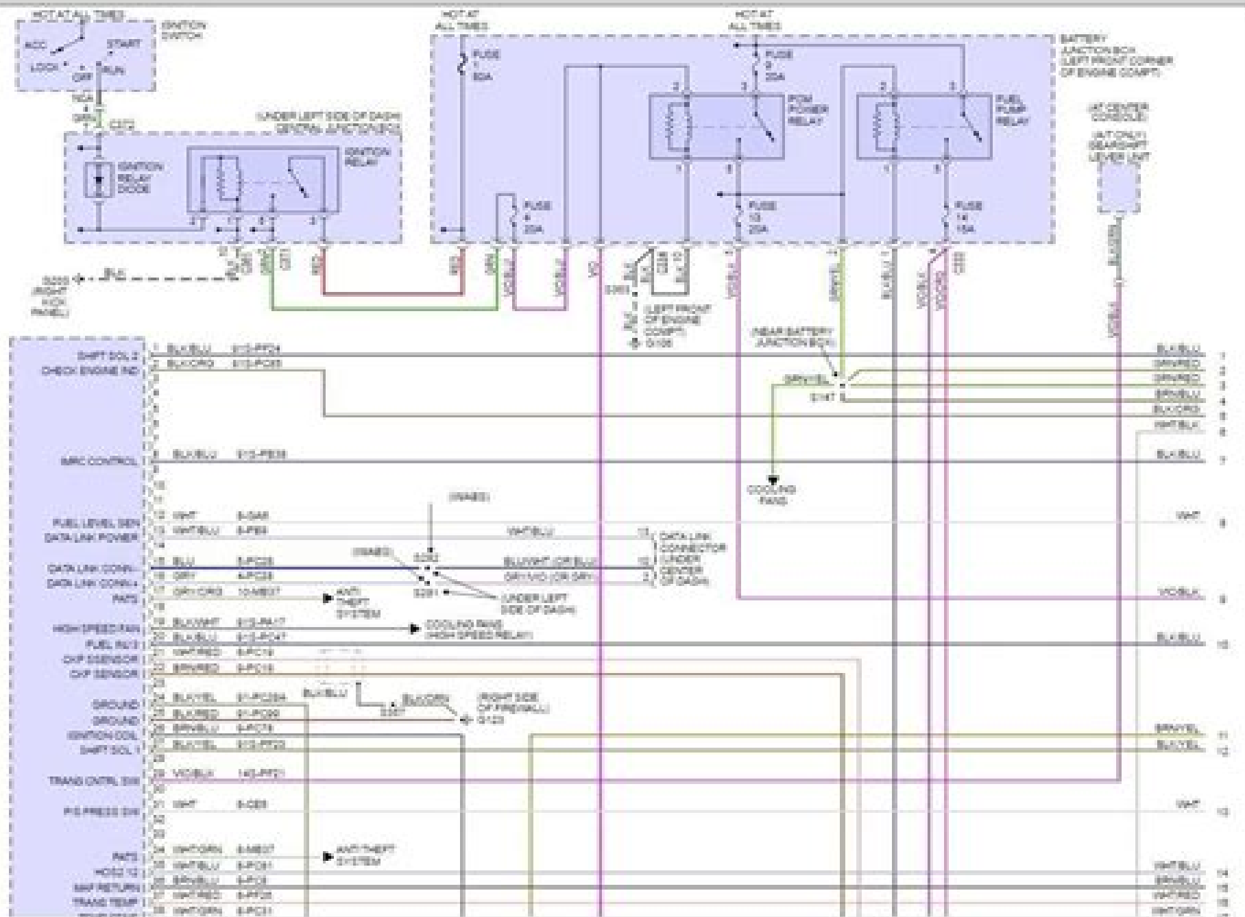
Fig 1: 2.5L, Engine Performance Circuit, Early Production (1 of 3)
