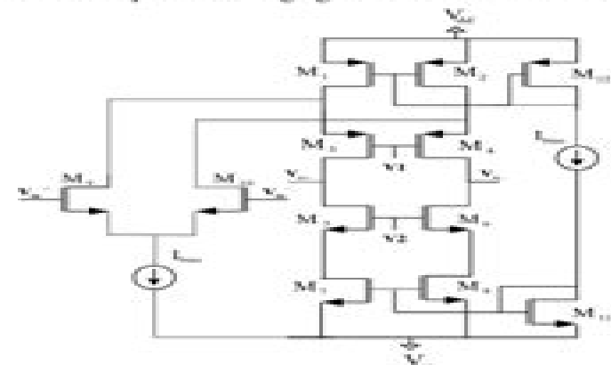
Fig. 1 Folded cascode OTA topology
