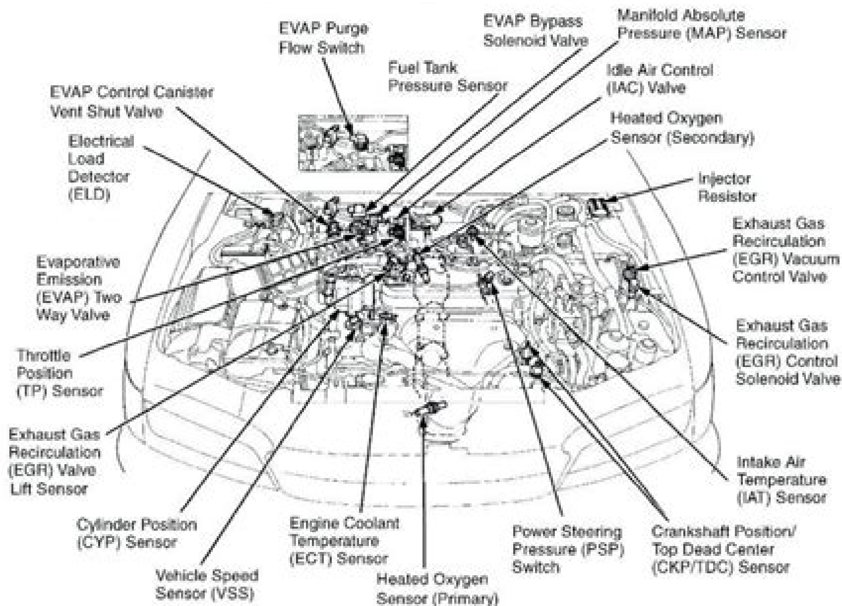
Fig. 5: Engine Compartment (1996) (2.2L)
