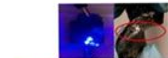
Magnetic force & interaction
