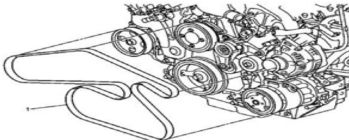
Fig. 1: Identifying Drive Belt Routing Courtesy of GENERAL MOTORS COMPANY
