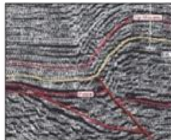
Seismic reflection
