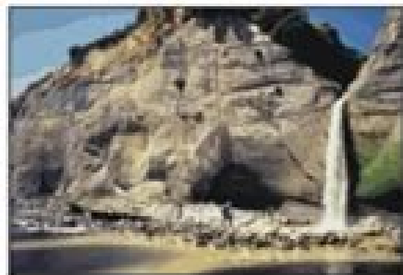
Outcrops
