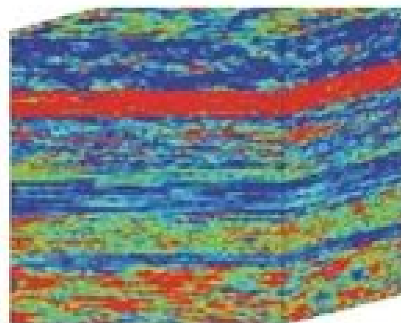
Computer 3D geologic models
