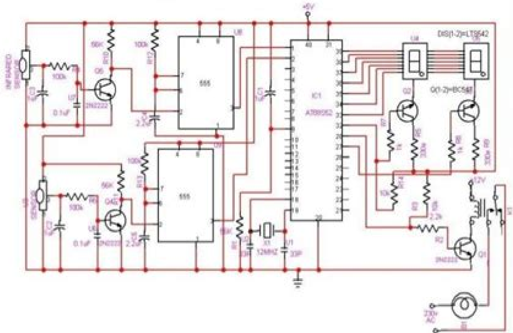
Receiver Circuit
