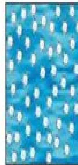
Colloidal solution
