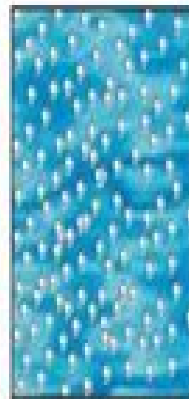
True solution
