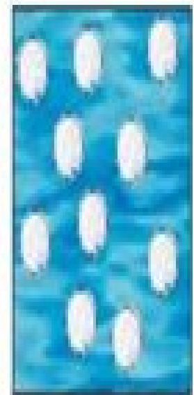
Suspensions
