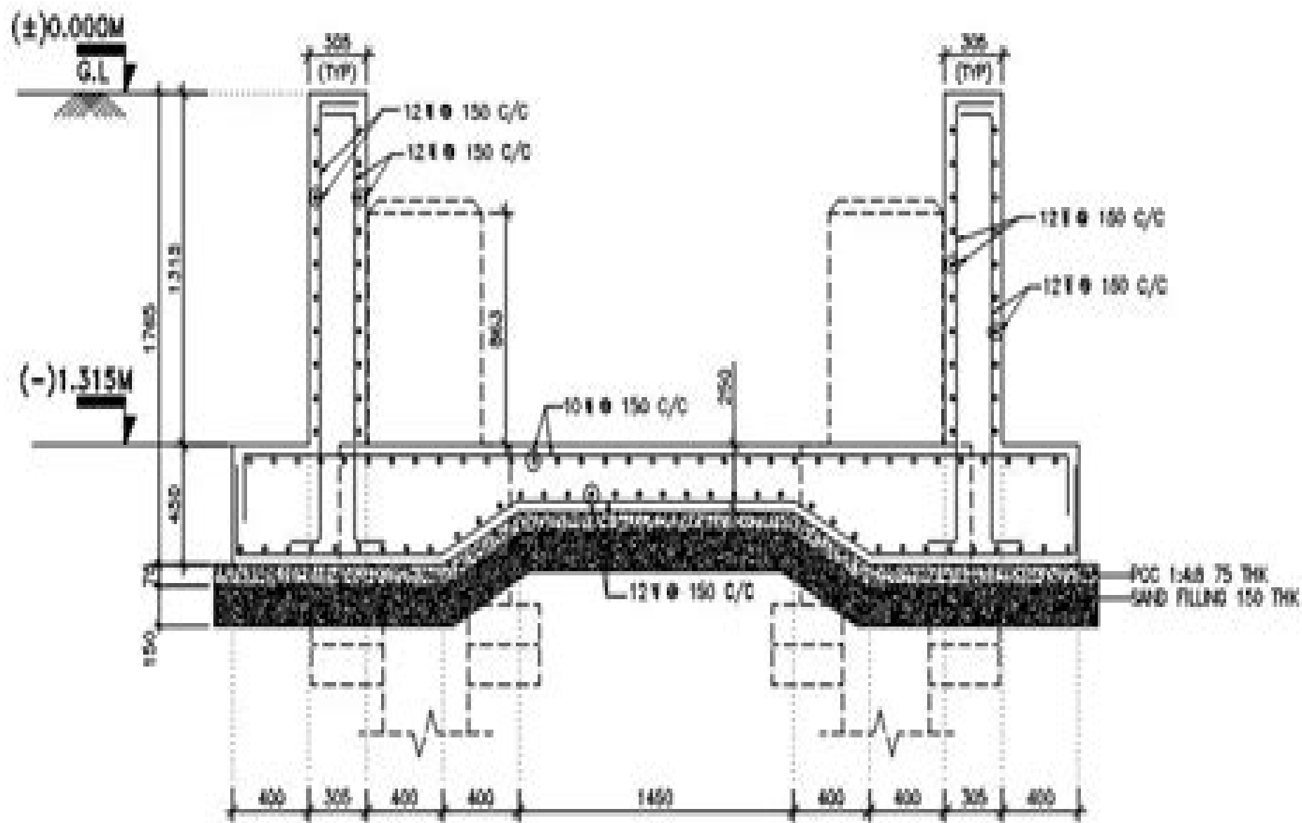
SECTION 4-4
