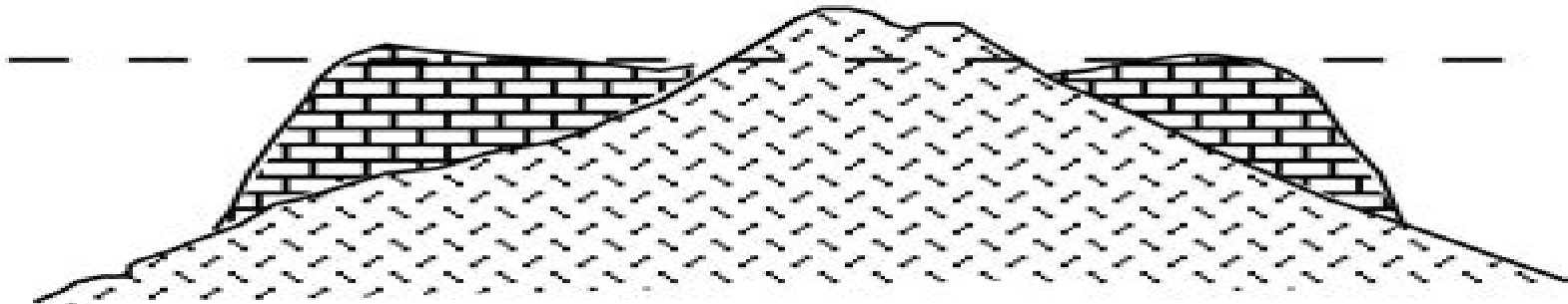
b) Barrier reef
