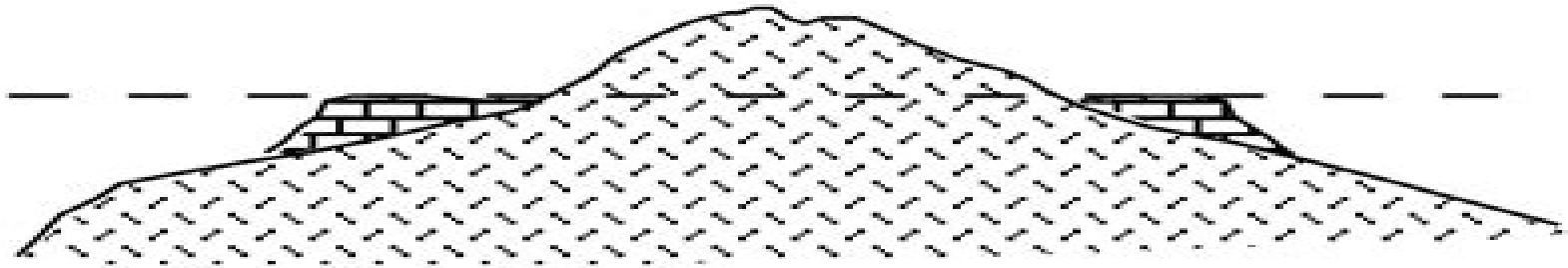
a) Fringing reef
