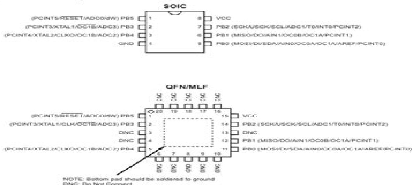
Figure 1. Pinout ATtiny25/45/85
