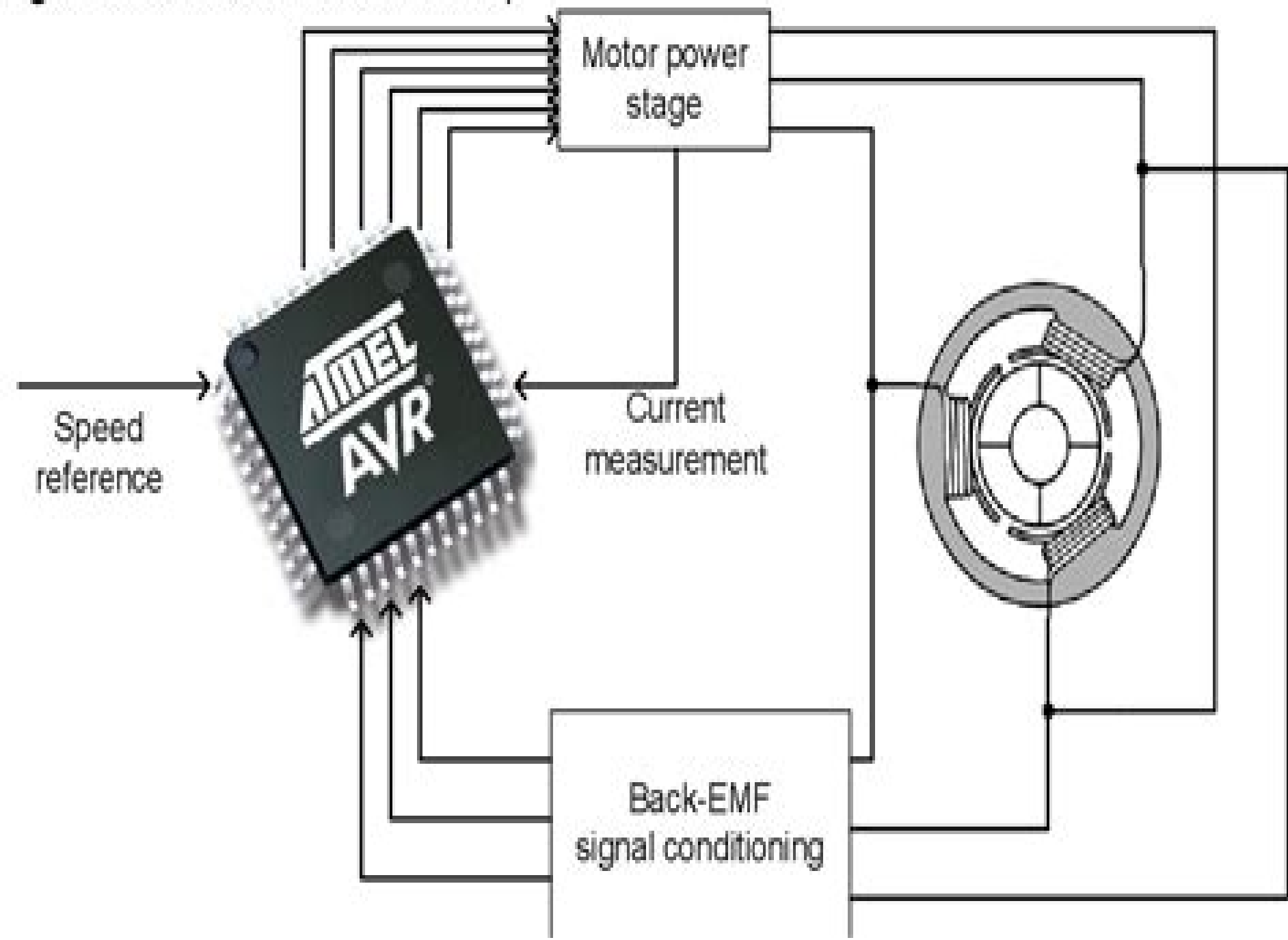
Figure 3. Sensorless control setup
