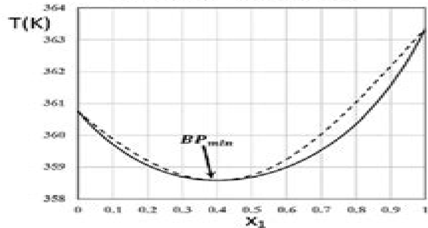
DMC(1) - sec-butyl formate(2)
