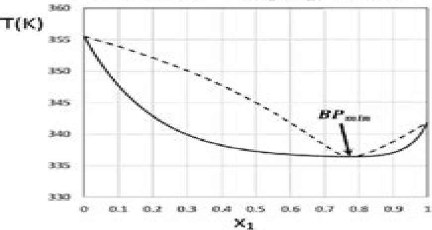
DMC(1) - isopropyl acetate(2)
