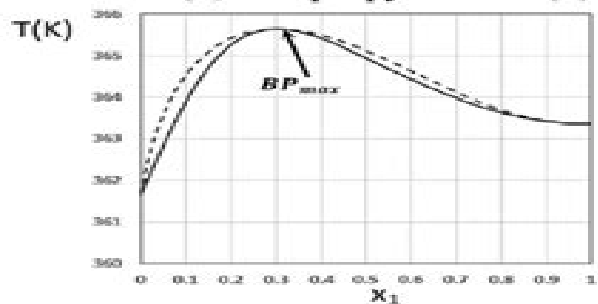
DMC(1) - methyl isobutyrate (2)
