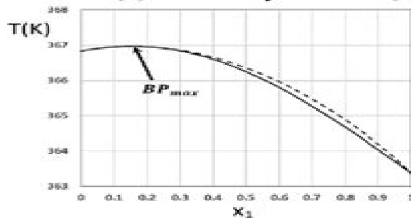
DMC(1) - butyl dimethyl amine (2)
