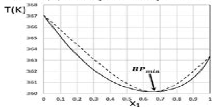
DMC(1) - butyl dimethyl amine (2)
