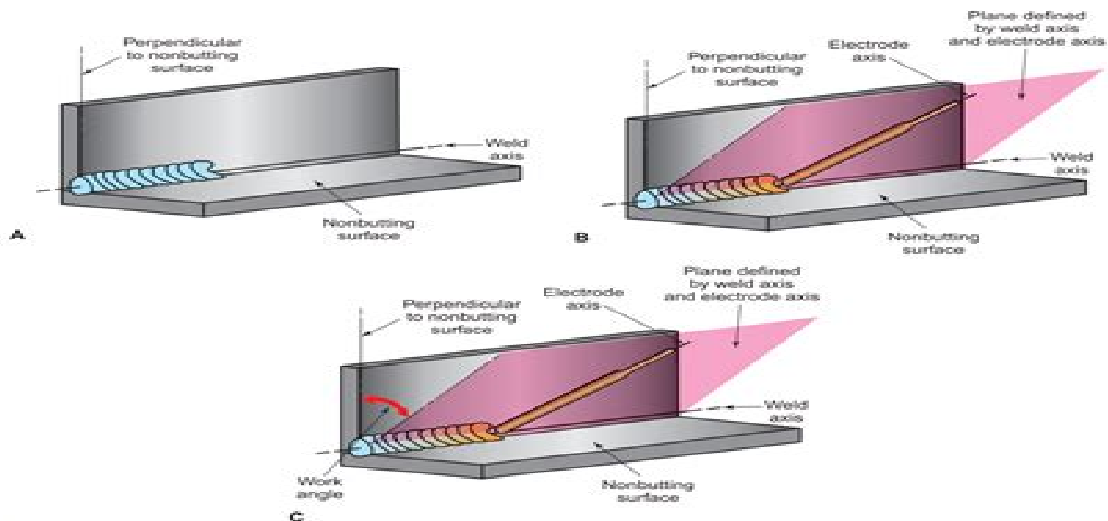
Figure 3-46. Work angle for an inside corner joint. The work angle is measured from a line perpendicular to the major or nonbutting surface to the plane containing the weld axis and the centerline of the electrode. A—The weld axis and a line perpendicular to the nonbutting surface are shown. B—The plane defined by the weld axis and the electrode axis are shown. C—The work angle is shown.
