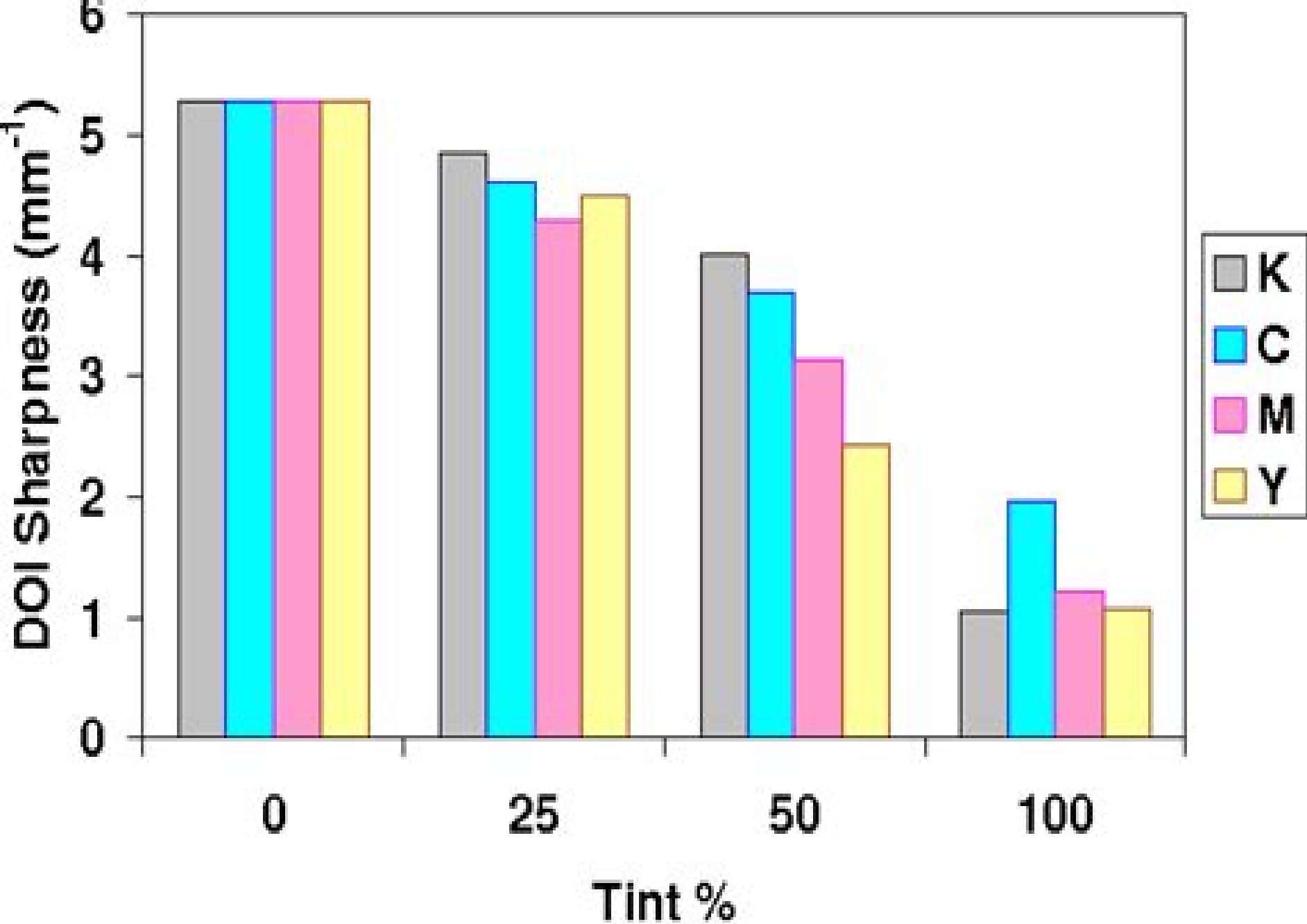
Fig 14a Effect of Tint % on DOI HP5500 on Paper 1
