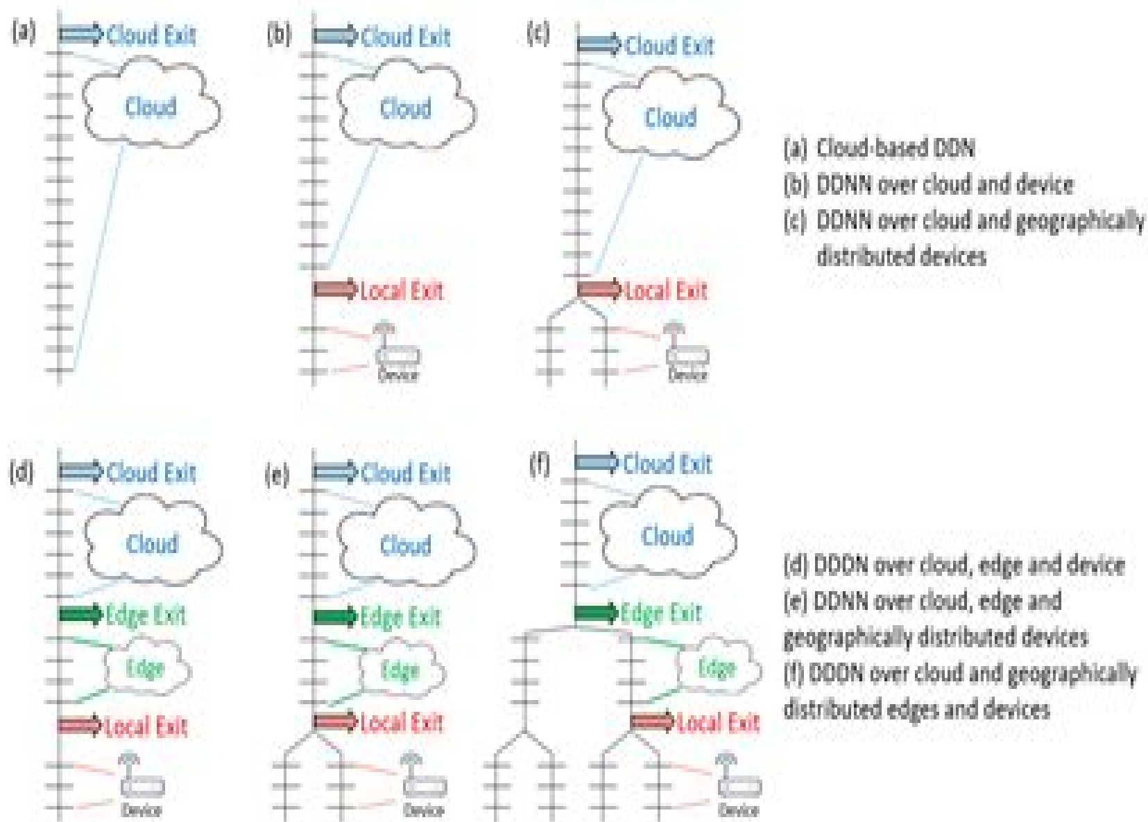
Figure 2. Overview of the DDNN architecture. The vertical lines represent the DNN pipeline, which connects the horizontal bars (NN layers). (a) is the standard DDN (processed entirely in the cloud), (b) introduces end devices and a local exit point that may classify samples before the cloud, (c) extends (b) by adding multiple end devices which are aggregated together for classification, (d) and (e) extend (b) and (c) by adding edge layers between the cloud and end devices, and (f) shows how the edge can also be distributed like the end devices.
