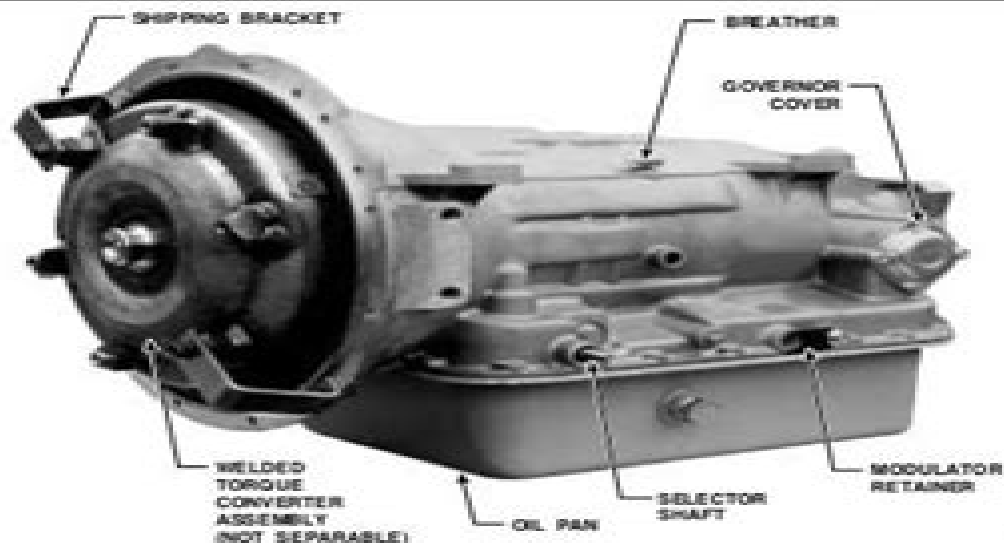
Figure 1-1. AT 154S Automatic Transmission — Left-Front View
