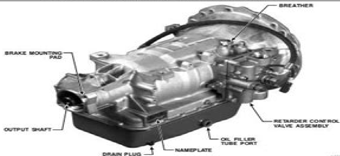
Figure 1-2. AT 54SR Automatic Transmission — Right-Rear View
