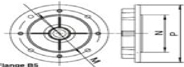
"D" Flange B5
