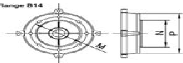
"C" Flange B14
