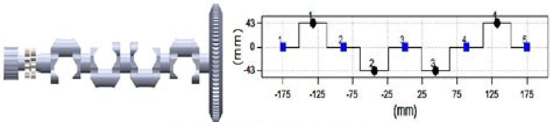
Fig. 2. The appearance torsional multi-mass model of the crankshaft
