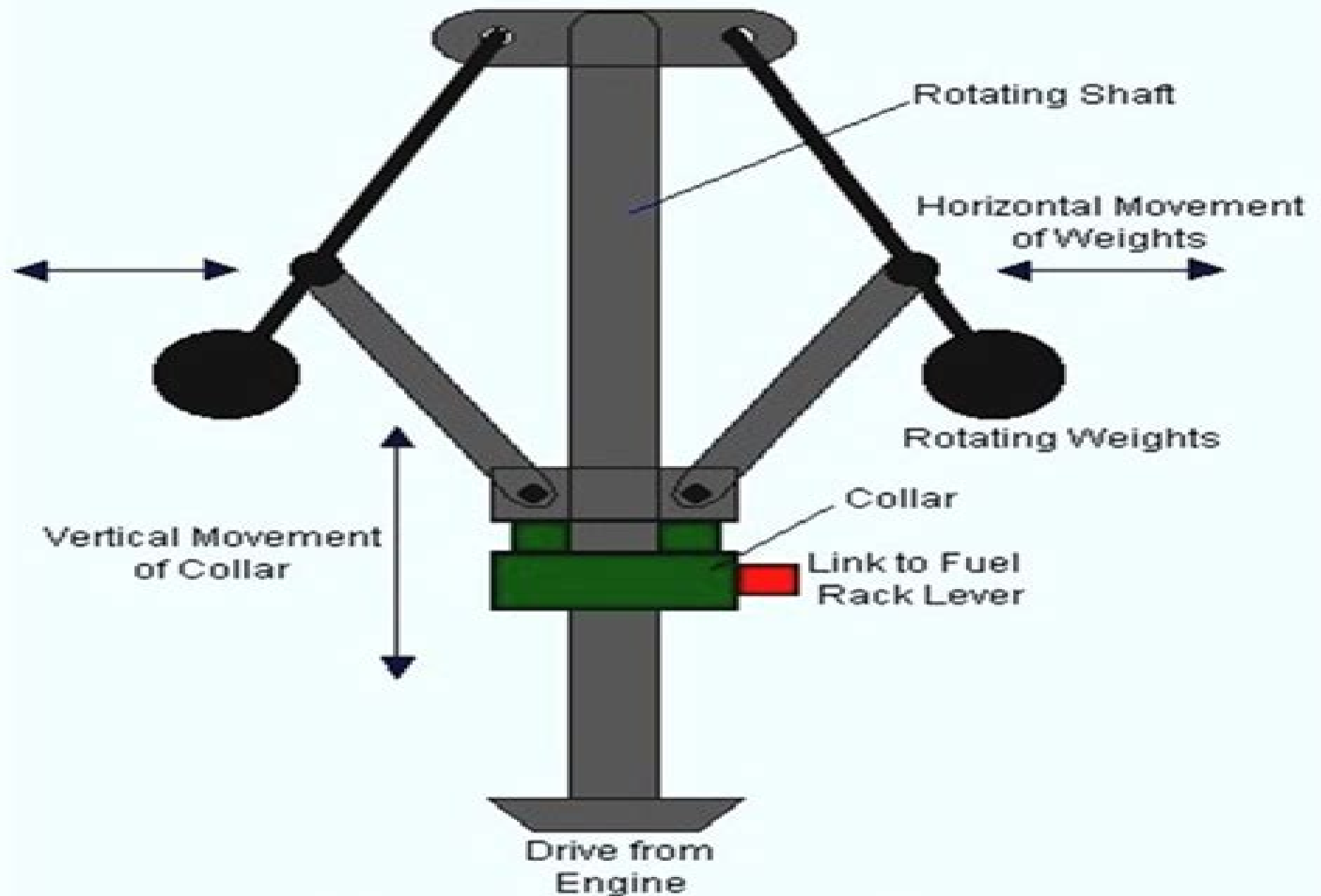
Engine Speed Governor
