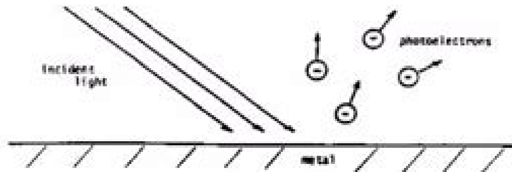
Figure 1. Light strikes a metallic surface and causes the emission of photoelectrons.
