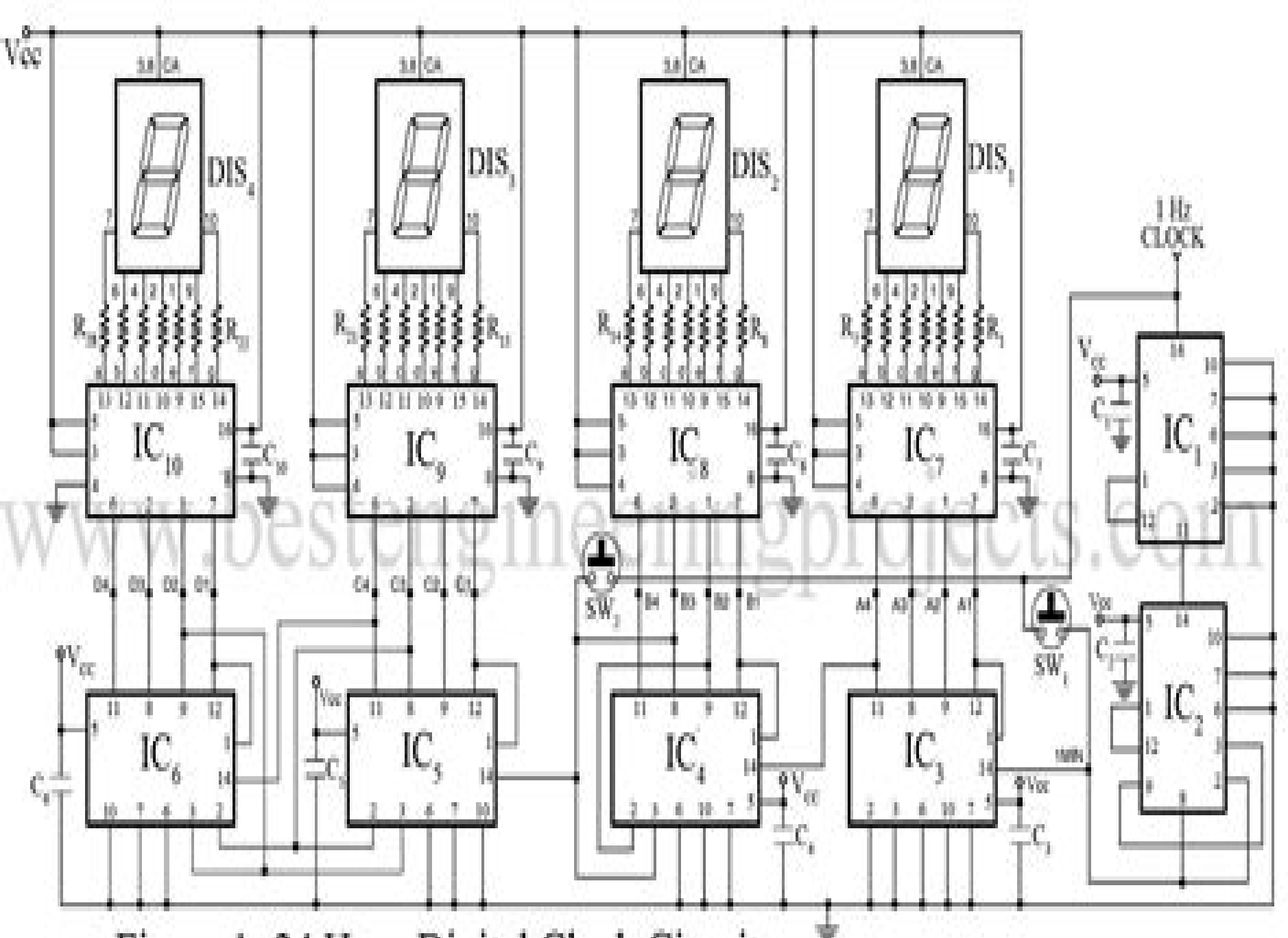
Figure 1: 24 Hour Digital Clock Circuit
