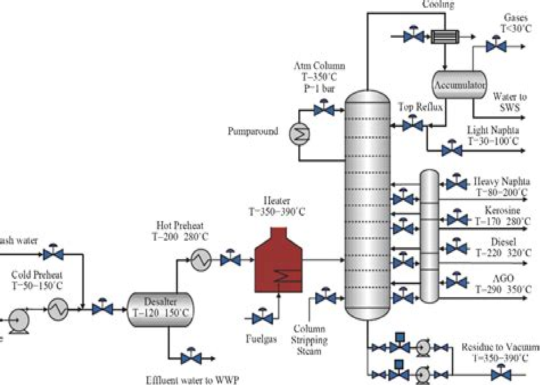
Figure 1. Process overview of crude oil distillation column.
