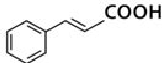
Cinnamic acid
