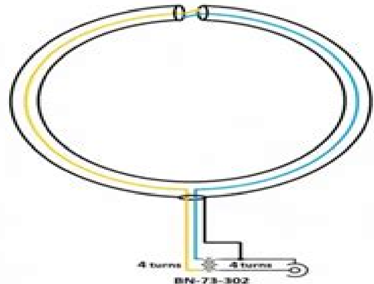
Passive LF/MF Antenna for Airspy HF+ Discovery
