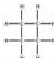
CYCLOBUTANE
