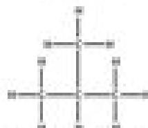
2-METHYL PROpane
