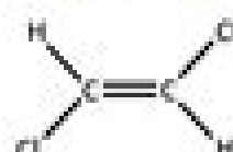
(E)-1,2-DICHLOROETHENE E = opposite side
