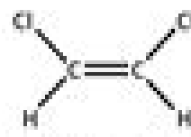
(Z)-1,2-DICHLOROETHENE Z = same side
