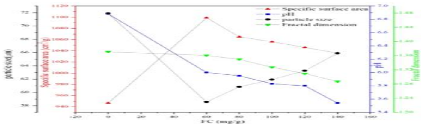
(b) Effect of FC on specific surface area, pH, fractal dimension and particle size
