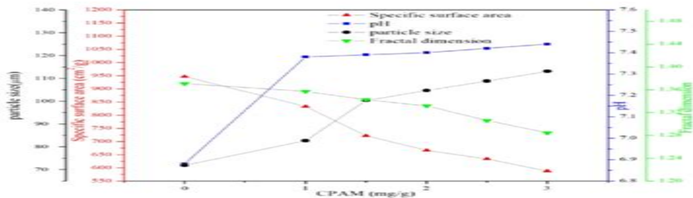
(c) Effect of CPAM on specific surface area, pH, fractal dimension and particle size
