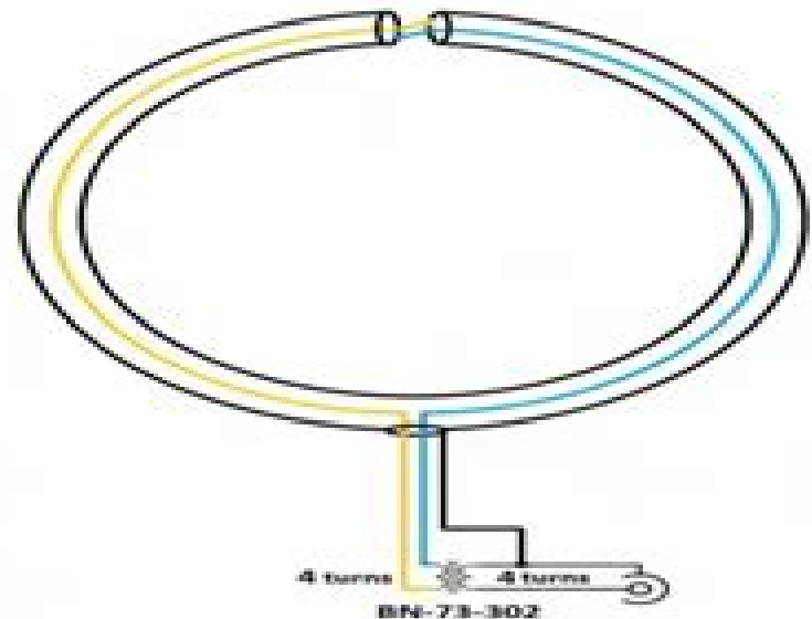
Passive LF/MF Antenna for Airspy HF+ Discovery
