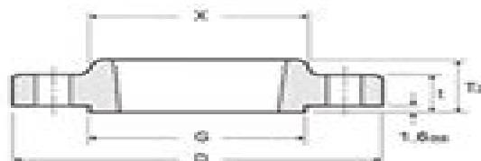
THREADED
