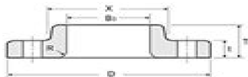
LAP JOINT
