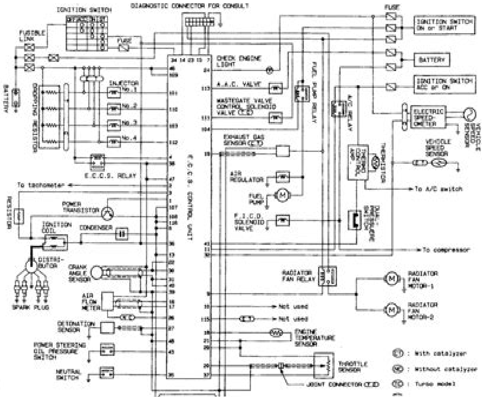
Circuit Diagram
