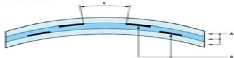
Figure 2. Diagram detailing clearance and creepage distance requirements for thin-film insulation.
