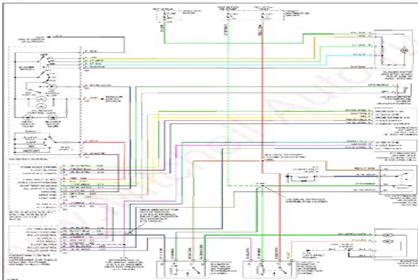
Fig. 1: Air Conditioning Circuits
