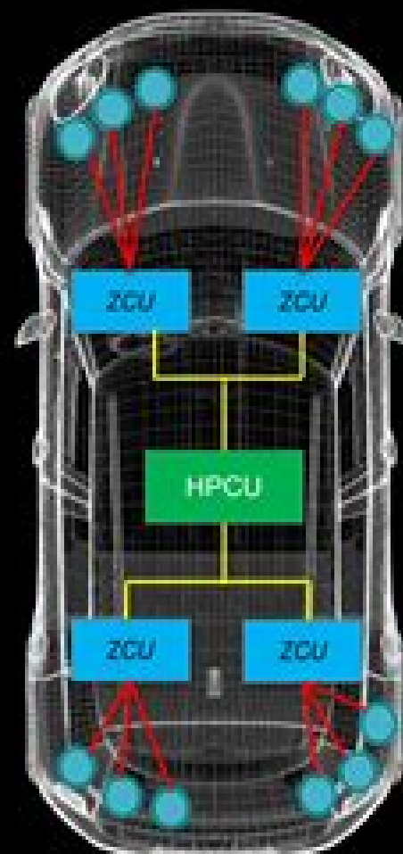
Zonal Architecture Zone CPUs handle all tasks within a certain physical area
