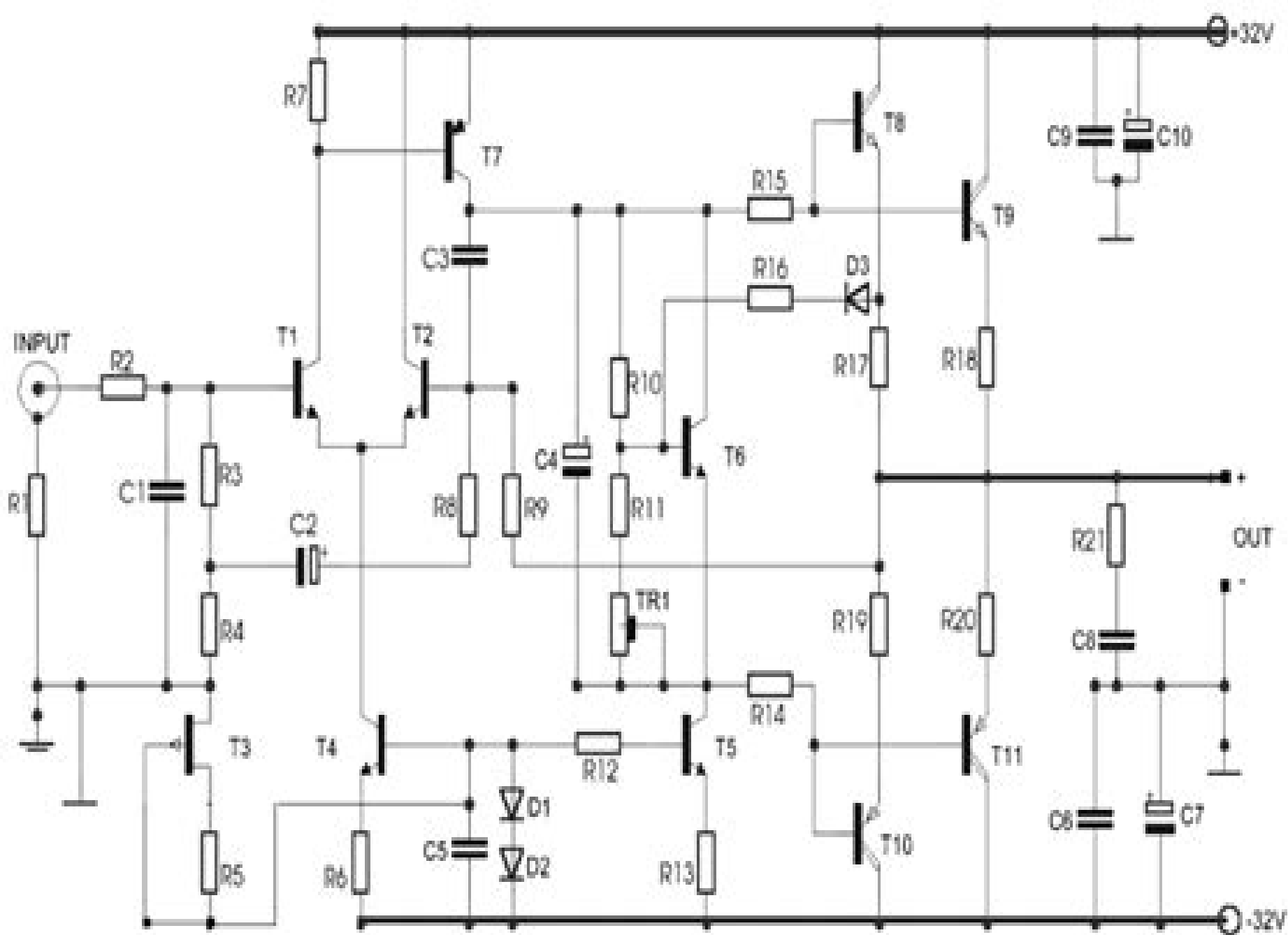
POWER AMPLIFIER 40W-Class A
