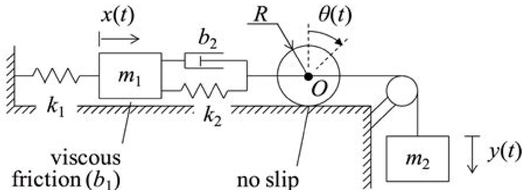
Figure 1. Three-Body System
