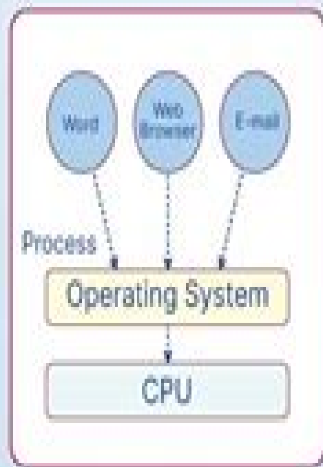
Multi-tasking
