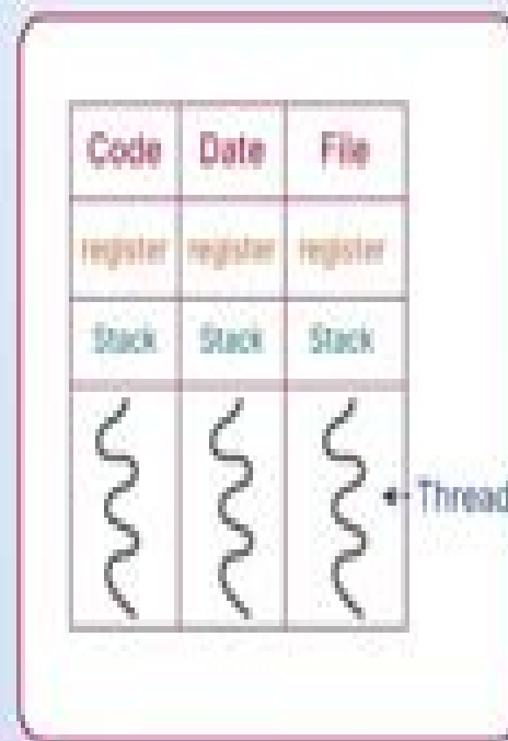
Multi-threading
