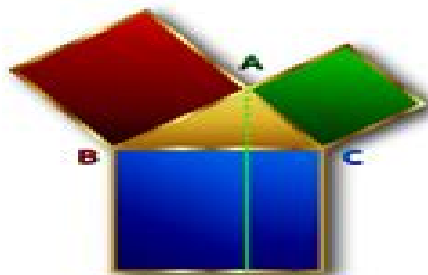
Euclid's Proof of the Pythagorean Theorem
